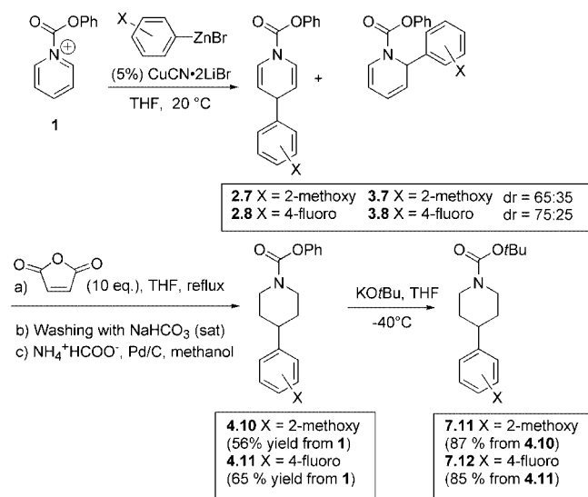
Scheme 1. Synthesis of isomerically pure 4-substituted piperidines 7.11 and 7.12 by scavenging of the 2-substituted isomer by a [4+2] cycloaddition reaction with maleic anhydride followed by washing with NaHCO 3 (sat.)
